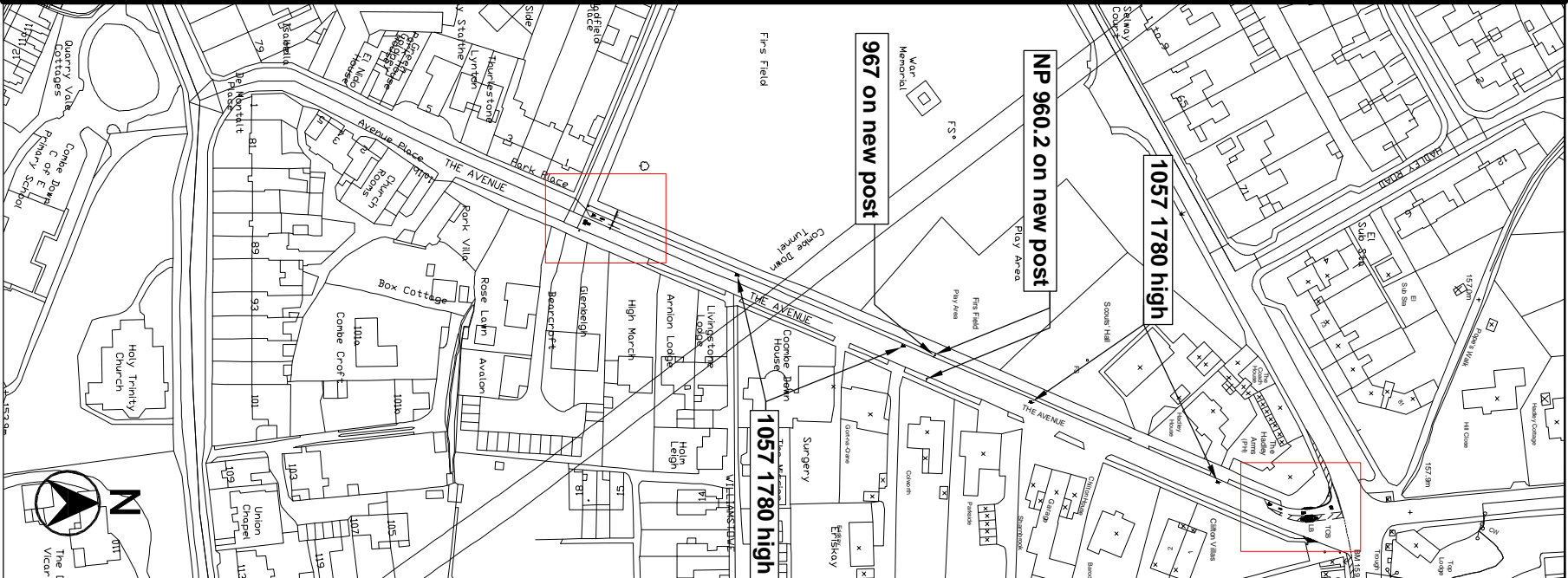
Location Plan 1:2000
